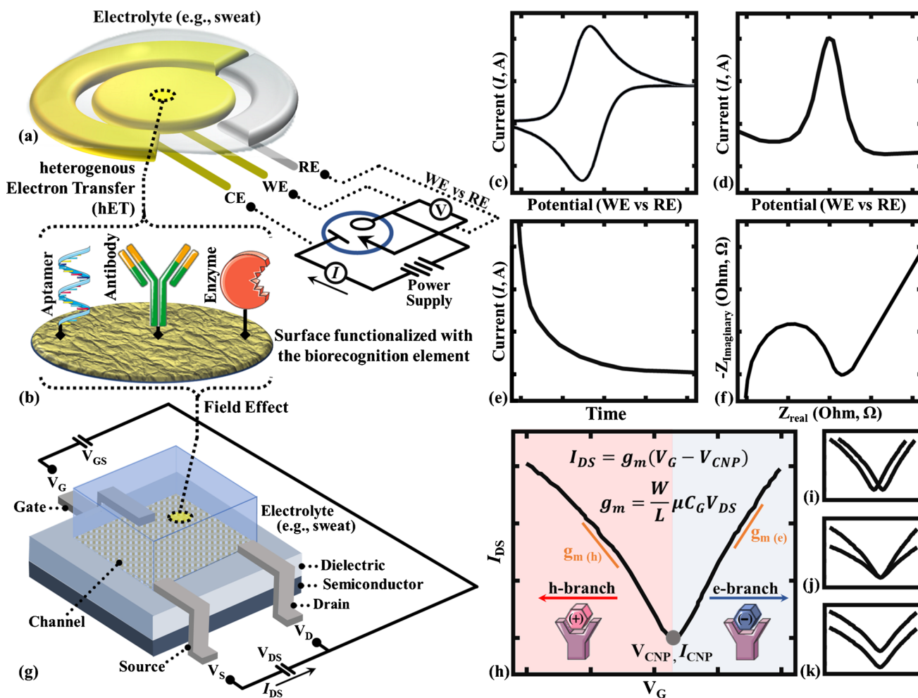
Fig. 3 Similar coplanar tripartite arrangement of wearable epidermal biosensors (WEBs) is applied in either electrochemical cells (a, c–f) or field-effect transistors (FETs); G–K). Commonly the screen-printed electrodes (SPEs) are used for WEBs (a), requiring reference (RE), working (WE), and counter (CE) electrodes. The assembly of a WEB implies the surface functionalization with a biorecognition element or receptor onto (b). Then the interaction with the analyte alters the electron transfer between the heterogeneous electrolyte–electrode interface mediated by a redox reaction that is recorded. The applied potential (V) comes from a potentiostat, i.e., power supply, being tuned between RE and WE. Commonly, the current (I) is recorded by cyclic voltammetry (c) and differential pulse voltammetry (d). Chronoamperometry is done at fixed potential for rapid measurements (e). Finally, electrochemical cells also can operate under a capacitive approach through the electrochemical impedance spectroscopy (EIS) (f). The detection region of FETs (g), is comprised by the source (S), drain (D) and gate (G) electrodes connected by a channel made of a
